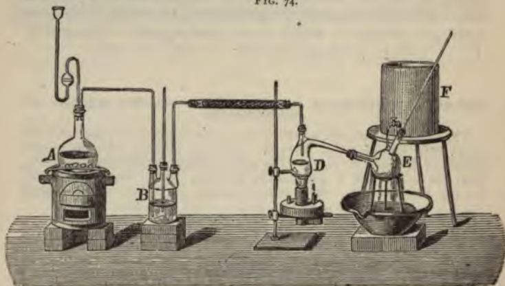
Phosphorus Trichloride—Phosphorous Chloride— \text{PCl}_3 . Conduct dry chlorine gas over phosphorus gently heated in
